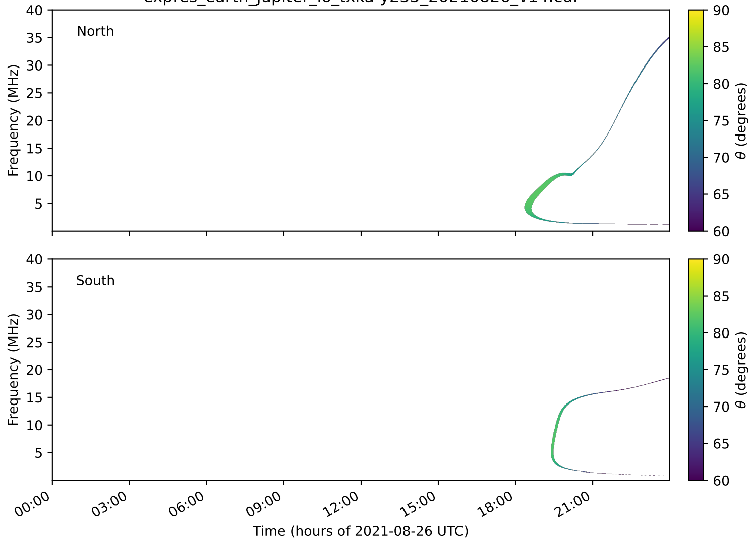
expres_earth_jupiter_io_txka-y235_20210826_v14.cdf
