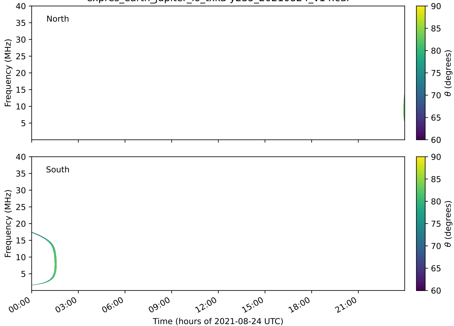
expres_earth_jupiter_io_txka-y235_20210824_v14.cdf
