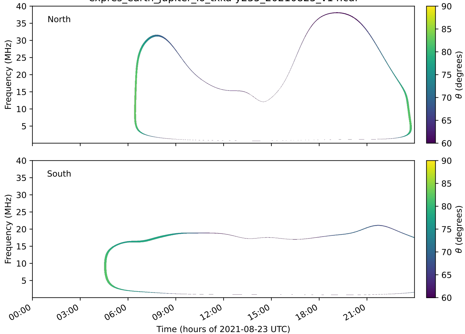
expres_earth_jupiter_io_txka-y235_20210823_v14.cdf
