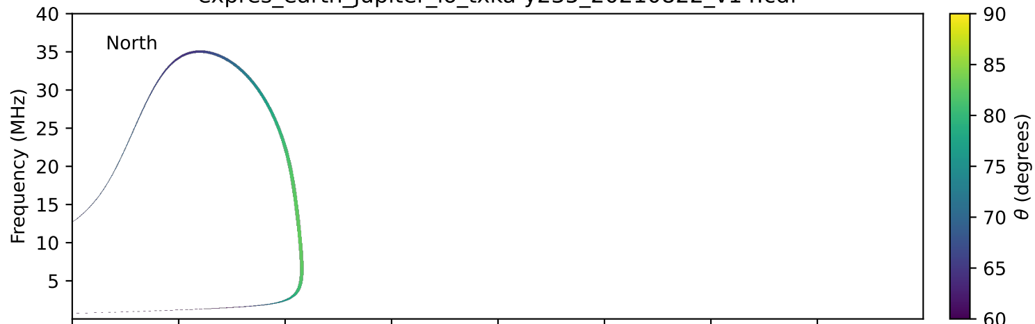
expres_earth_jupiter_io_txka-y235_20210822_v14.cdf
