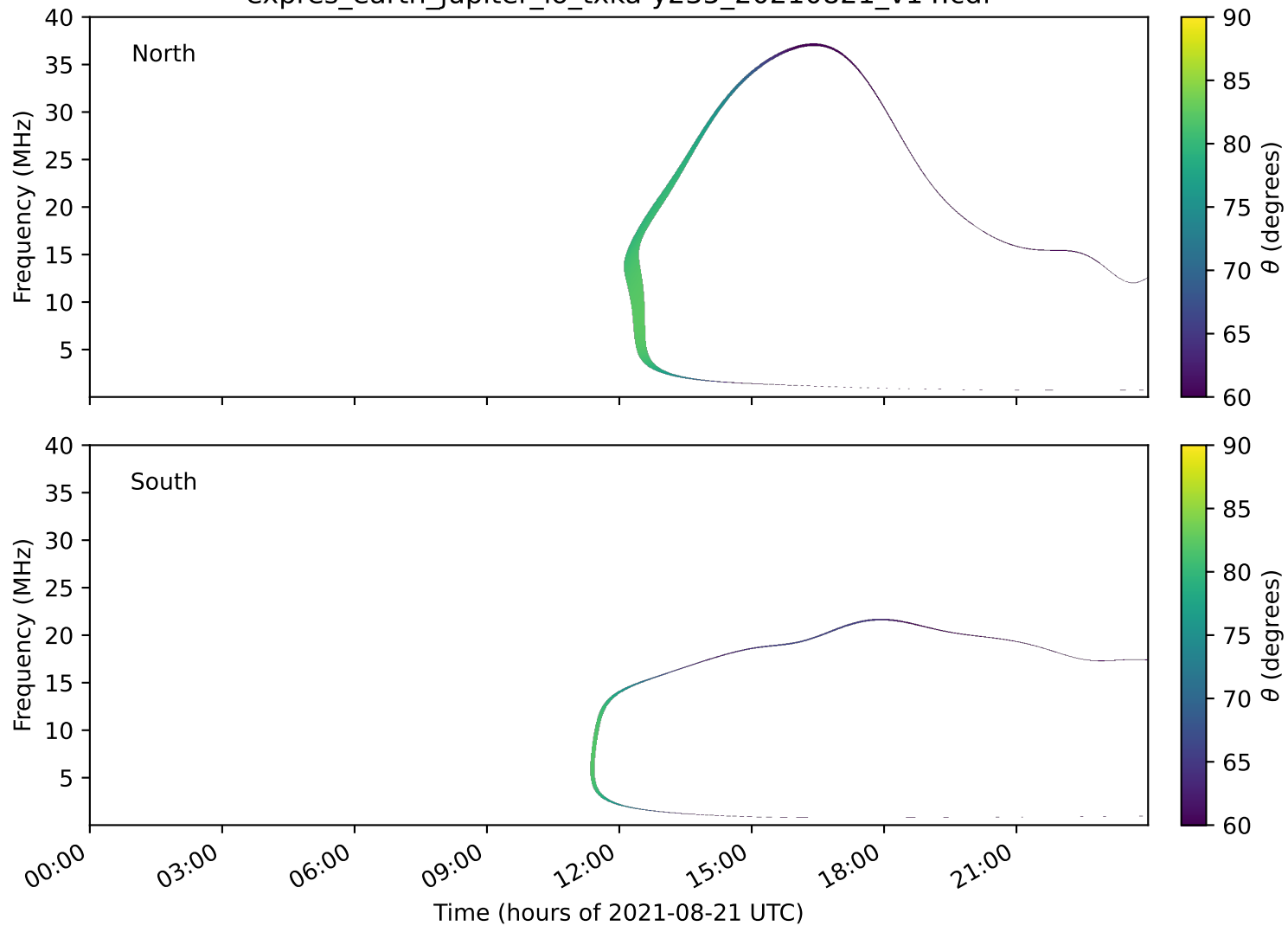
expres_earth_jupiter_io_txka-y235_20210821_v14.cdf
