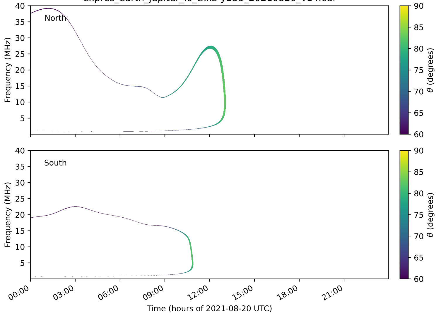
expres_earth_jupiter_io_txka-y235_20210820_v14.cdf
