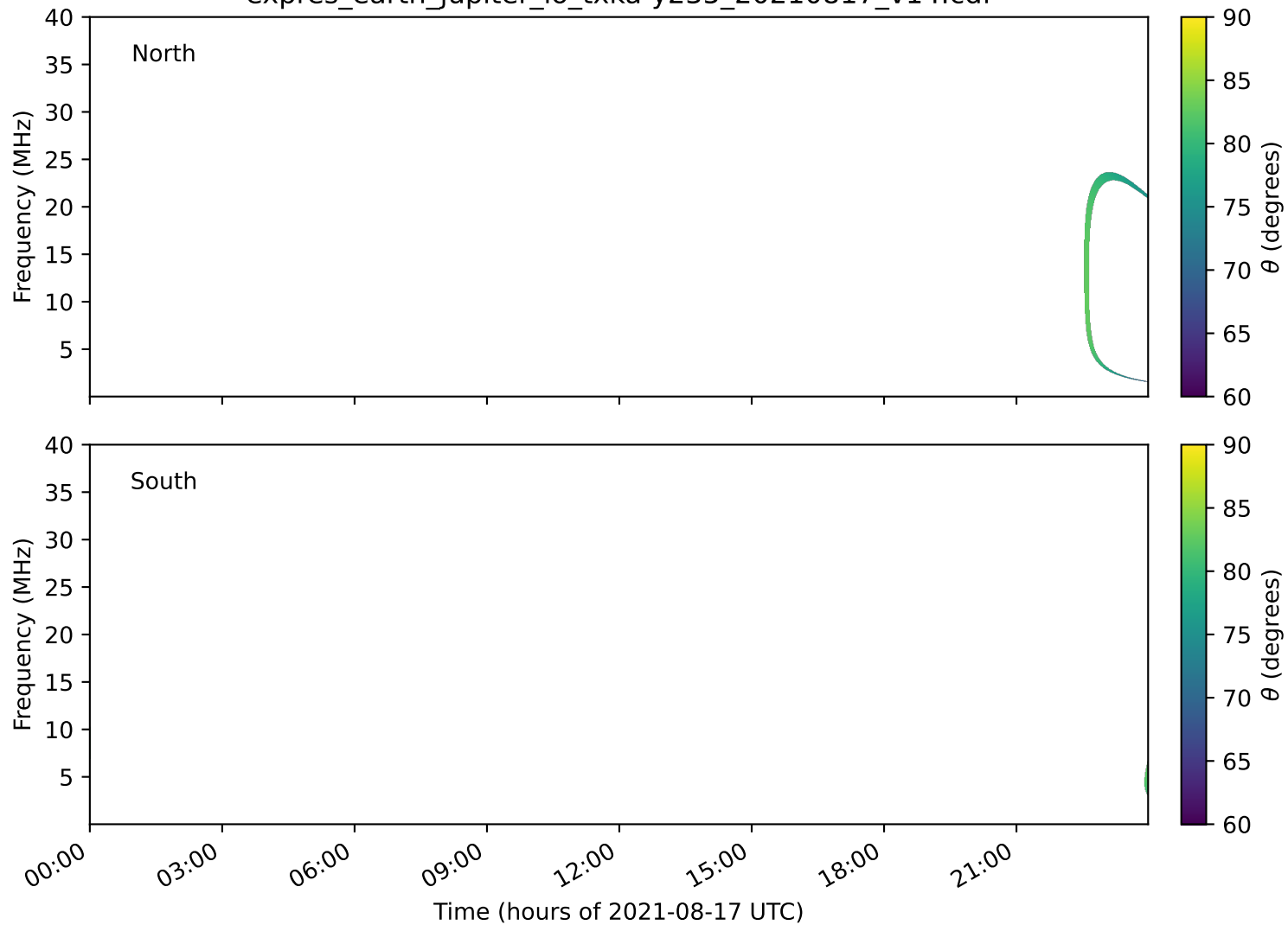
expres_earth_jupiter_io_txka-y235_20210817_v14.cdf
