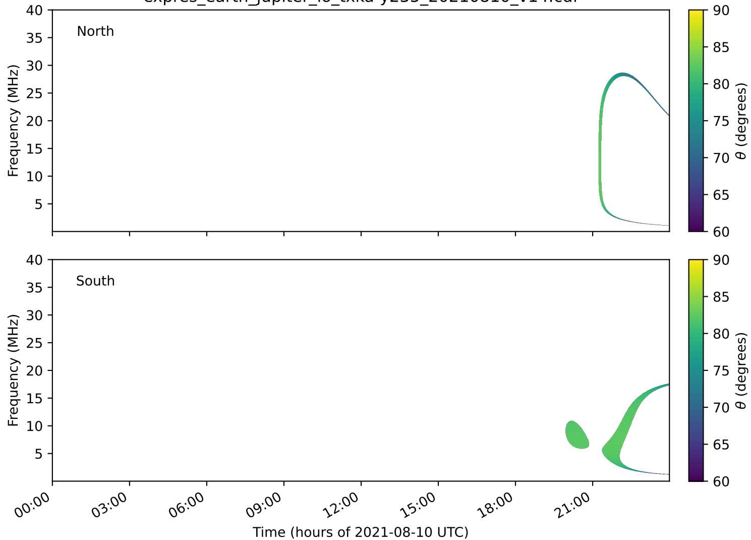
expres_earth_jupiter_io_txka-y235_20210810_v14.cdf
