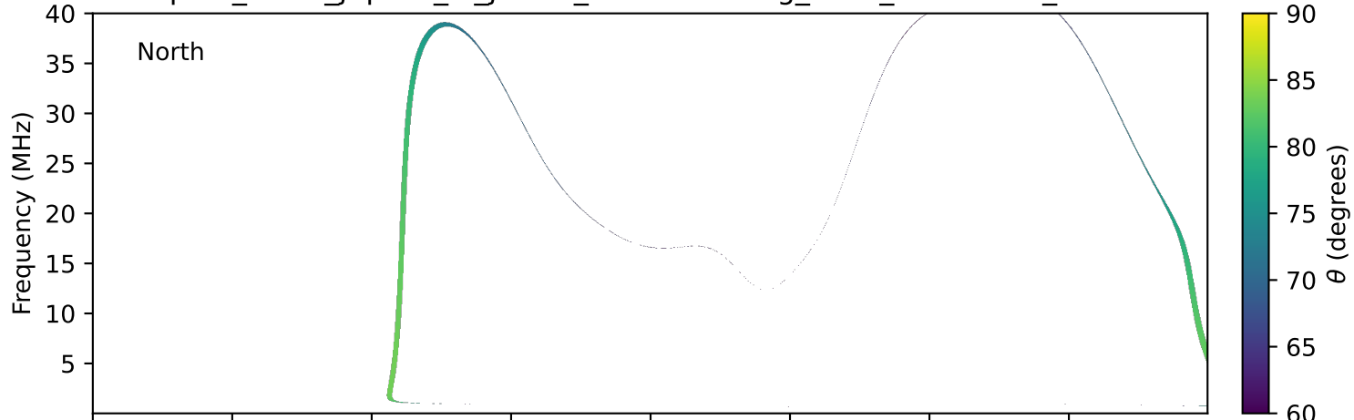
expres_earth_jupiter_io_jrm33_lossc-wid1deg_3kev_20210823_v11.cdf
