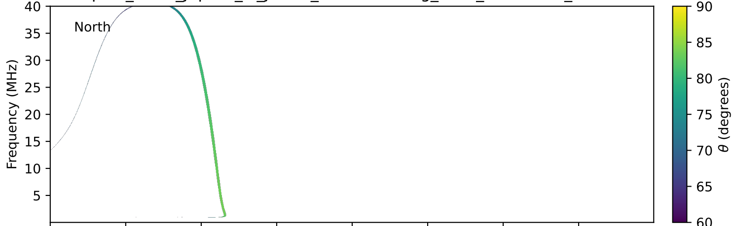
expres_earth_jupiter_io_jrm33_lossc-wid1deg_3kev_20210822_v11.cdf
