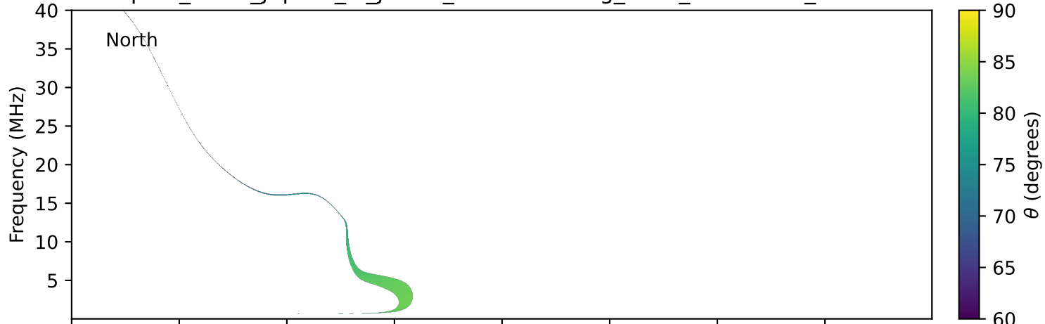
expres_earth_jupiter_io_jrm33_lossc-wid1deg_3kev_20210806_v11.cdf
