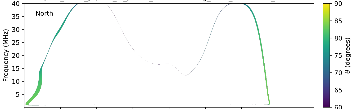
expres_earth_jupiter_io_jrm33_lossc-wid1deg_3kev_20210802_v11.cdf
