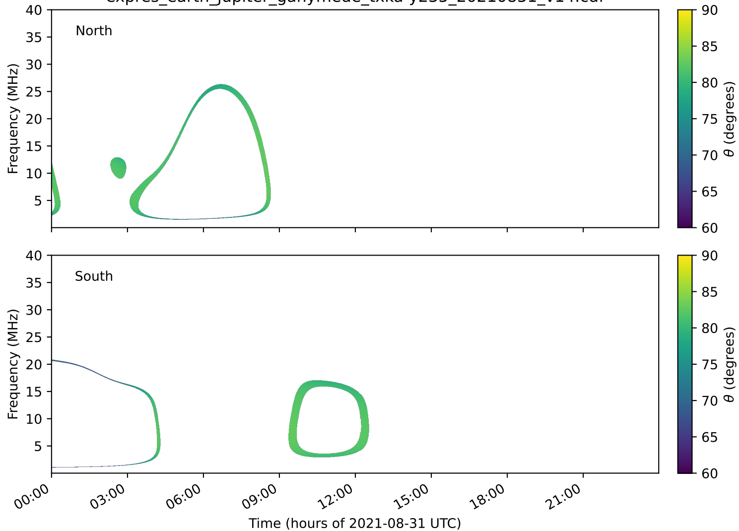
expres_earth_jupiter_ganymede_txka-y235_20210831_v14.cdf
