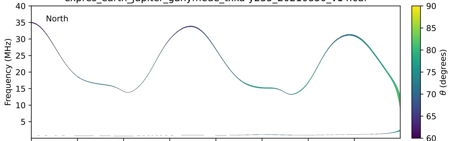
expres_earth_jupiter_ganymede_txka-y235_20210830_v14.cdf
