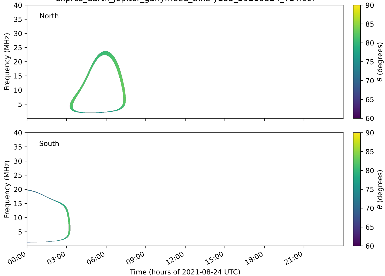
expres_earth_jupiter_ganymede_txka-y235_20210824_v14.cdf
