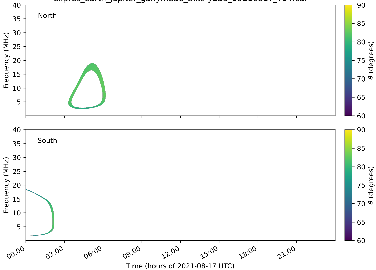
expres_earth_jupiter_ganymede_txka-y235_20210817_v14.cdf
