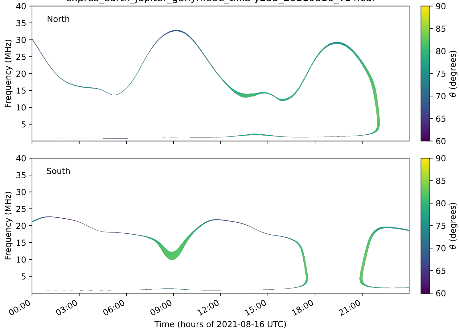
expres_earth_jupiter_ganymede_txka-y235_20210816_v14.cdf
