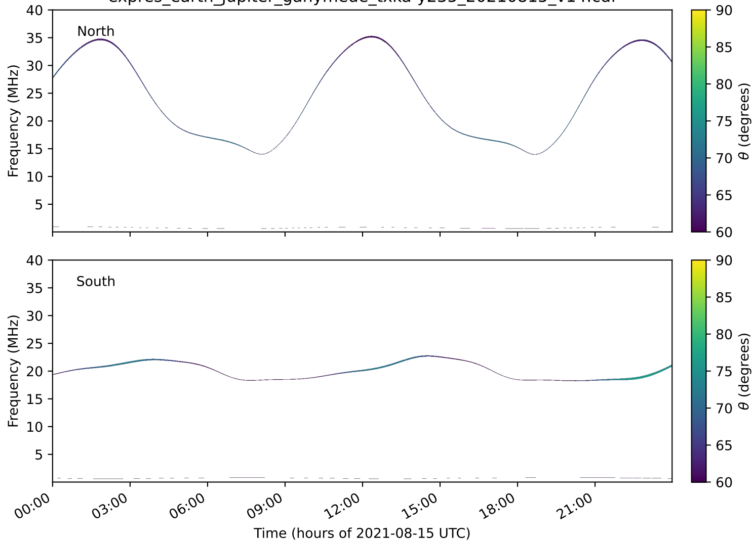
expres_earth_jupiter_ganymede_txka-y235_20210815_v14.cdf
