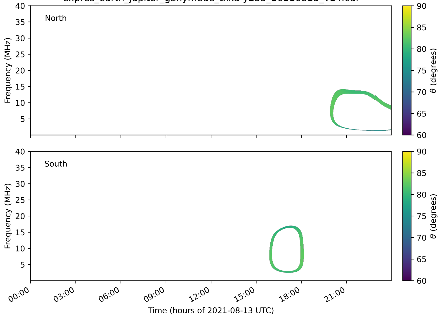
expres_earth_jupiter_ganymede_txka-y235_20210813_v14.cdf
