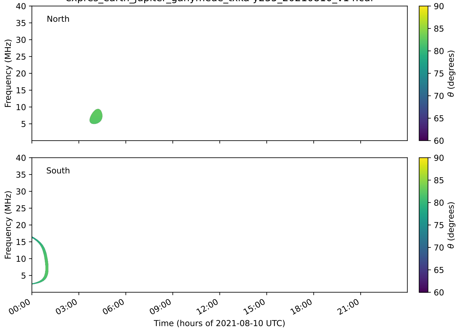
expres_earth_jupiter_ganymede_txka-y235_20210810_v14.cdf
