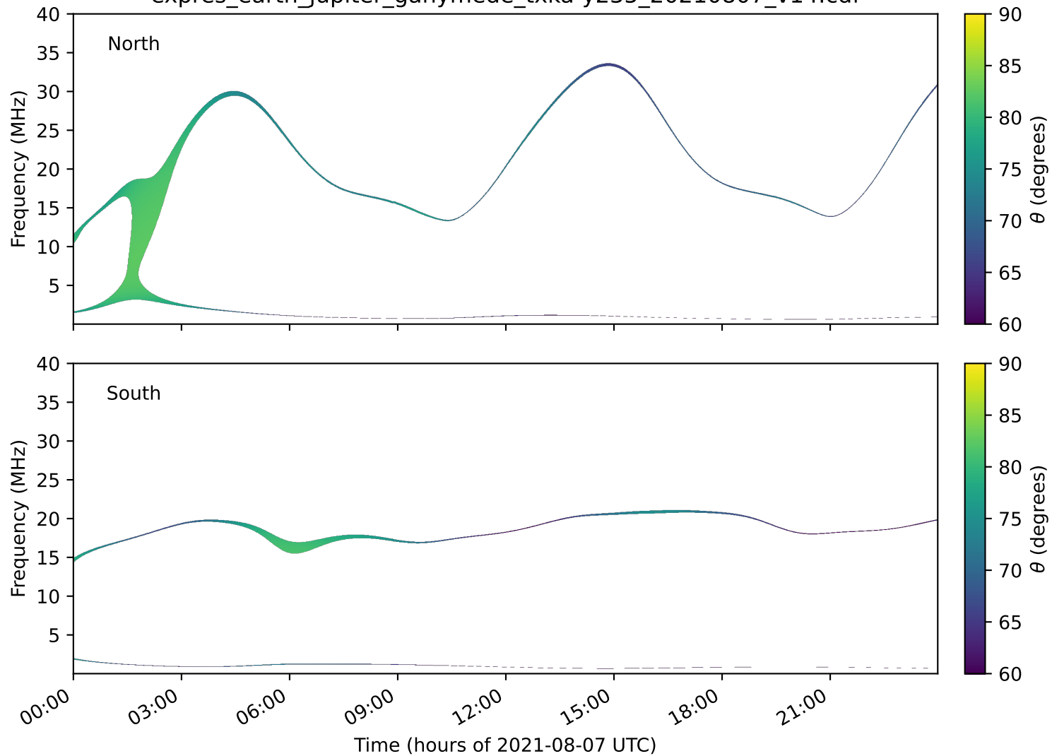
expres_earth_jupiter_ganymede_txka-y235_20210807_v14.cdf
