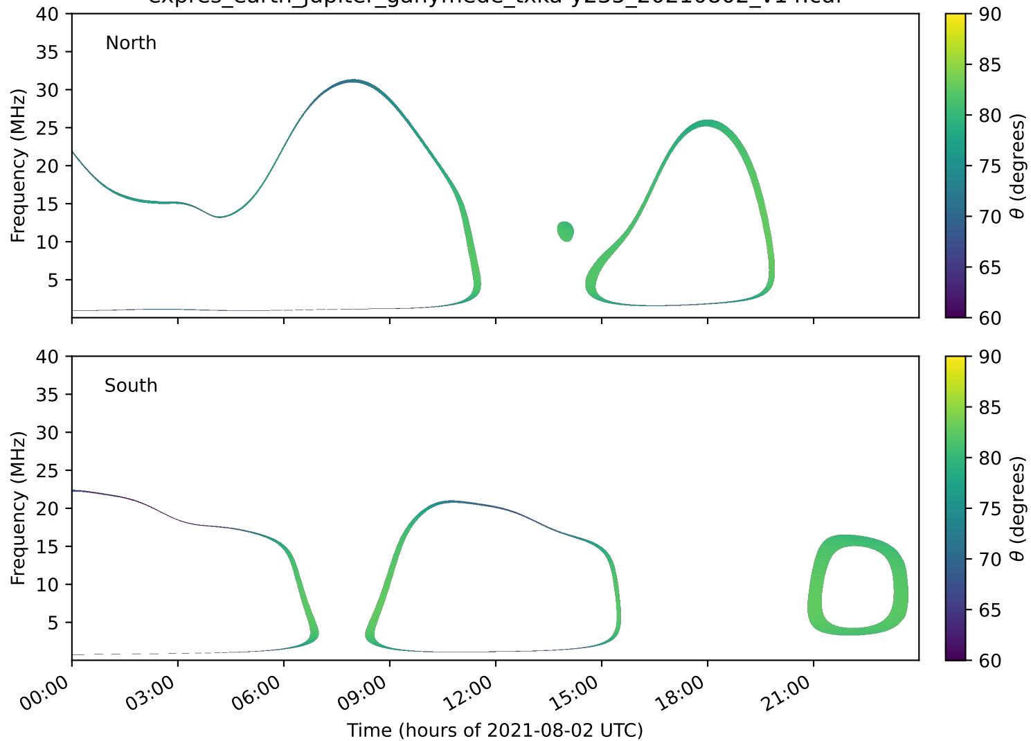
expres_earth_jupiter_ganymede_txka-y235_20210802_v14.cdf
