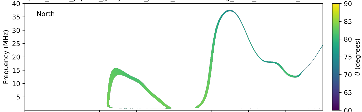
expres_earth_jupiter_ganymede_jrm33_lossc-wid1deg_3kev_20210828_v11.cdf
