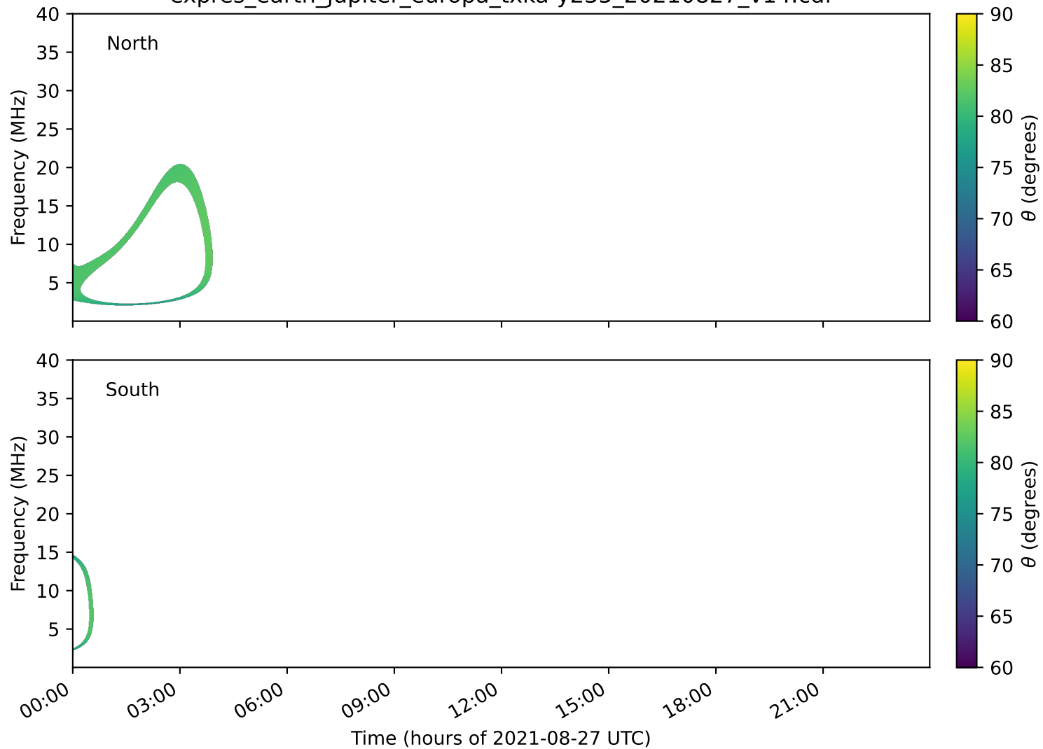
expres_earth_jupiter_europa_txka-y235_20210827_v14.cdf
