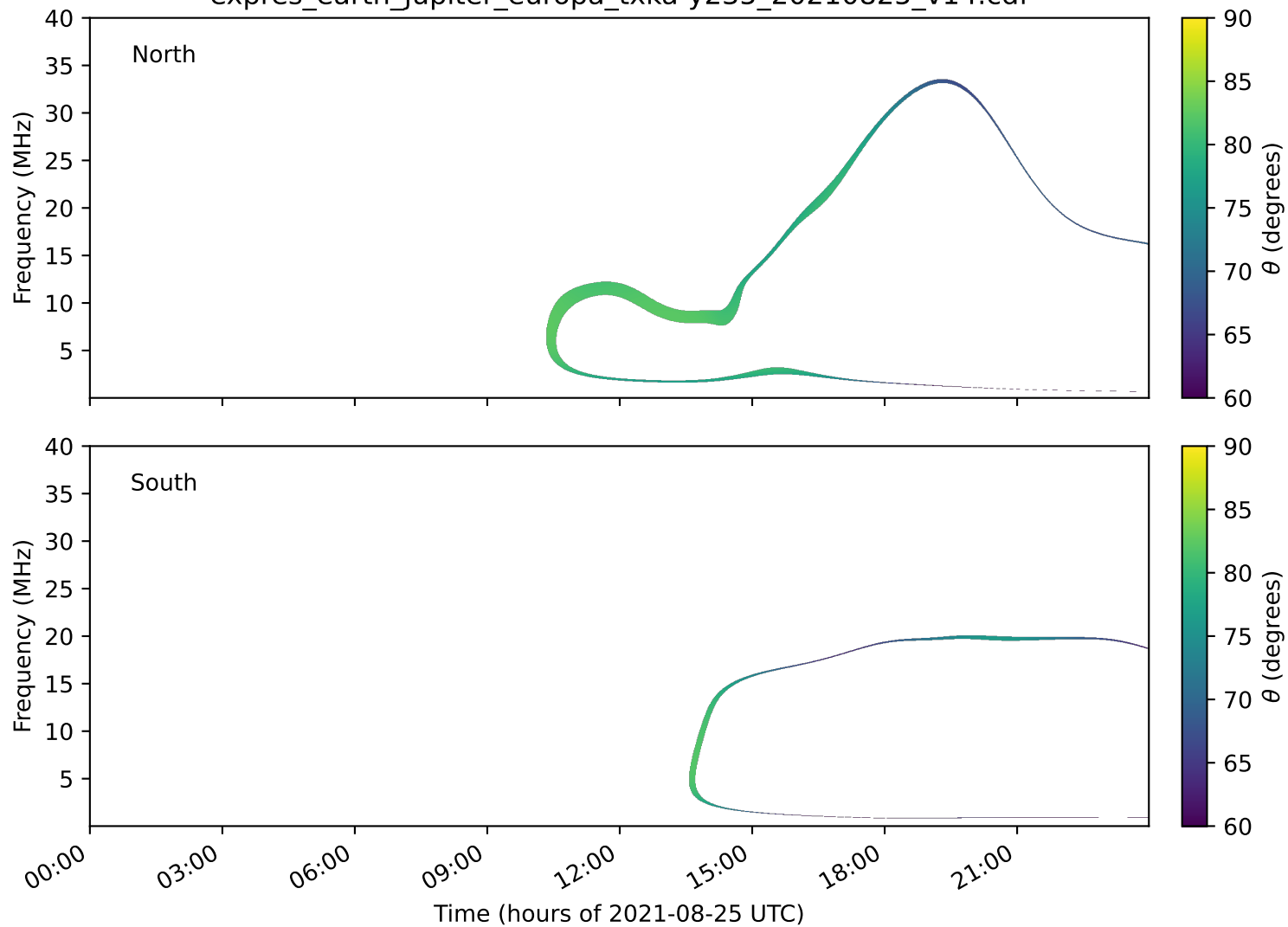
expres_earth_jupiter_europa_txka-y235_20210825_v14.cdf
