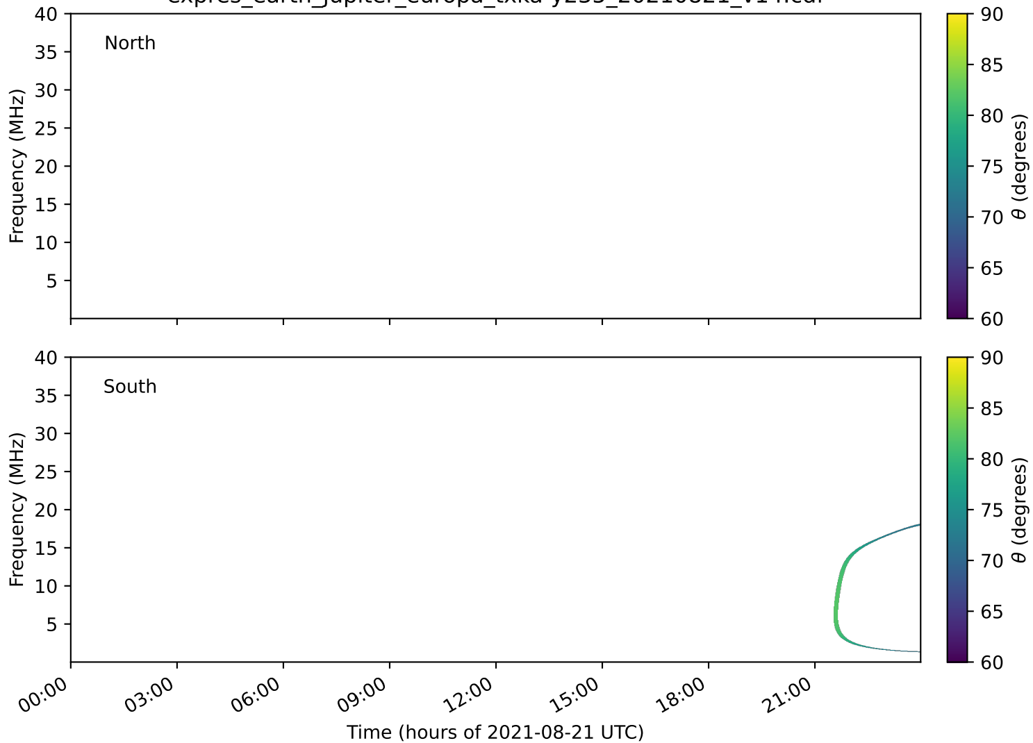
expres_earth_jupiter_europa_txka-y235_20210821_v14.cdf
