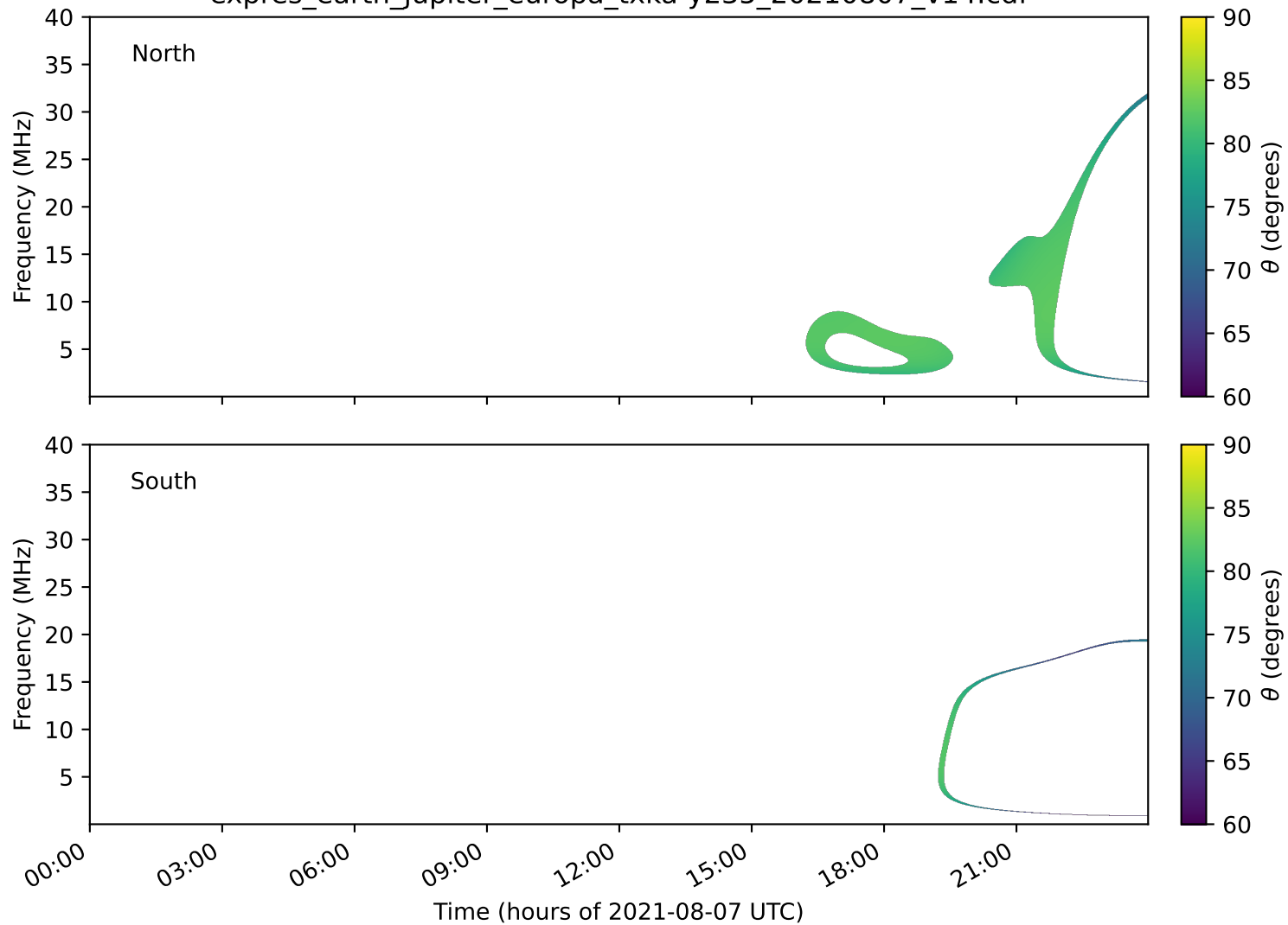
expres_earth_jupiter_europa_txka-y235_20210807_v14.cdf
