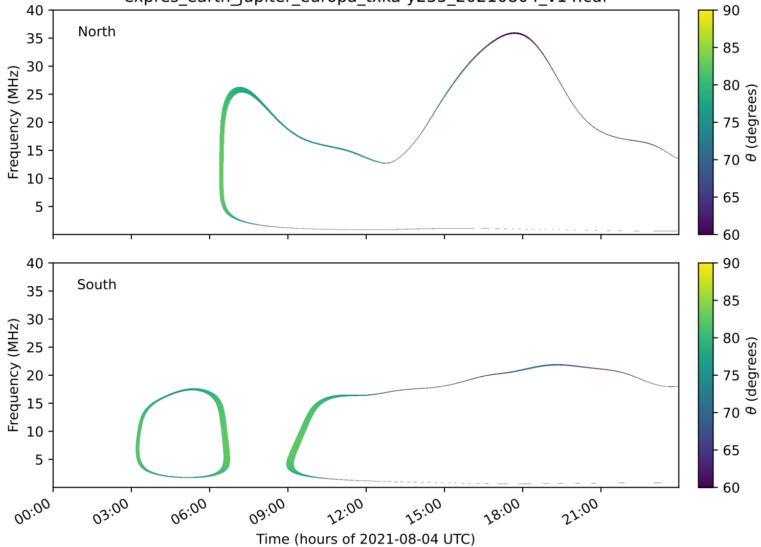
expres_earth_jupiter_europa_txka-y235_20210804_v14.cdf
