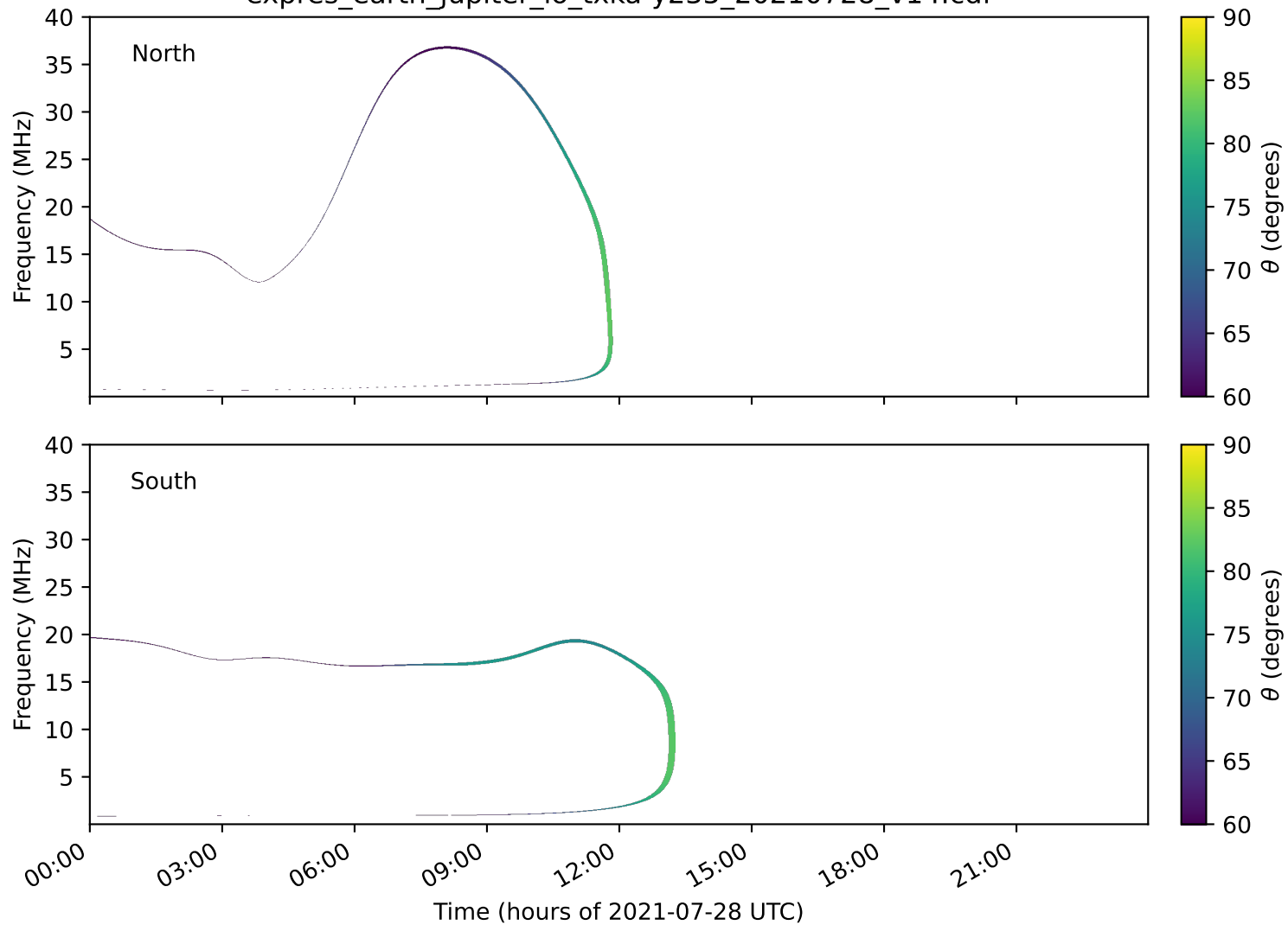
expres_earth_jupiter_io_txka-y235_20210728_v14.cdf
