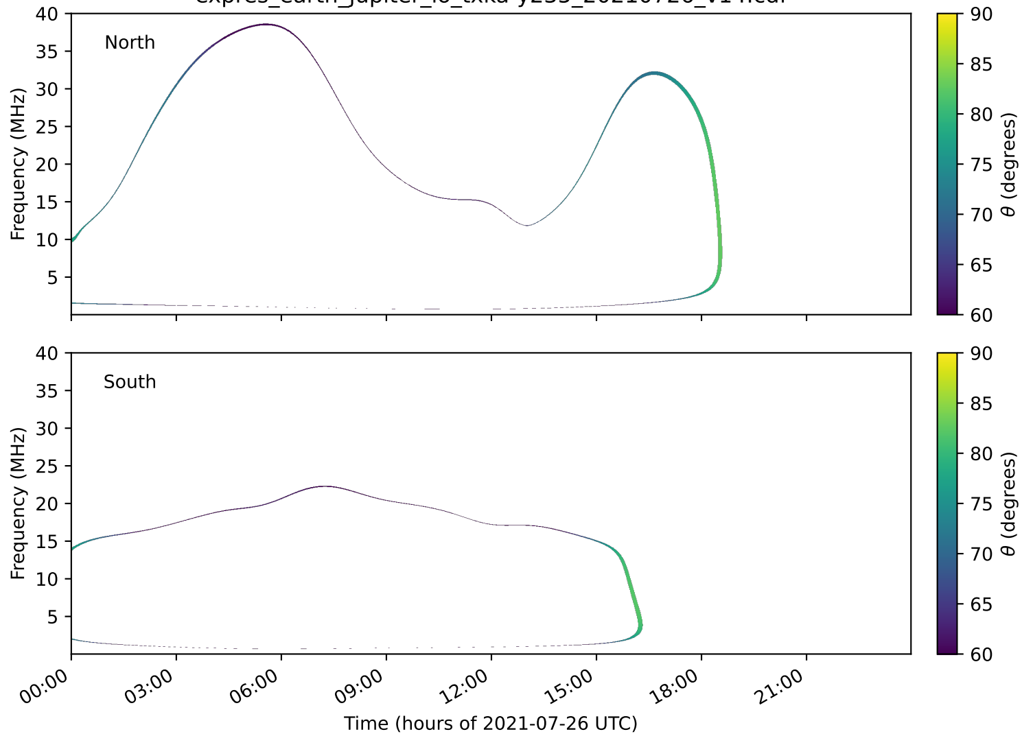
expres_earth_jupiter_io_txka-y235_20210726_v14.cdf
