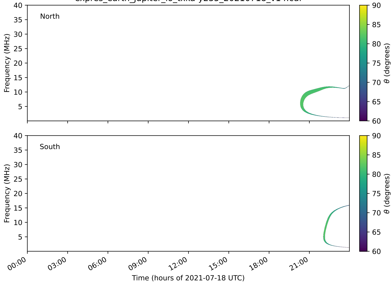
expres_earth_jupiter_io_txka-y235_20210718_v14.cdf
