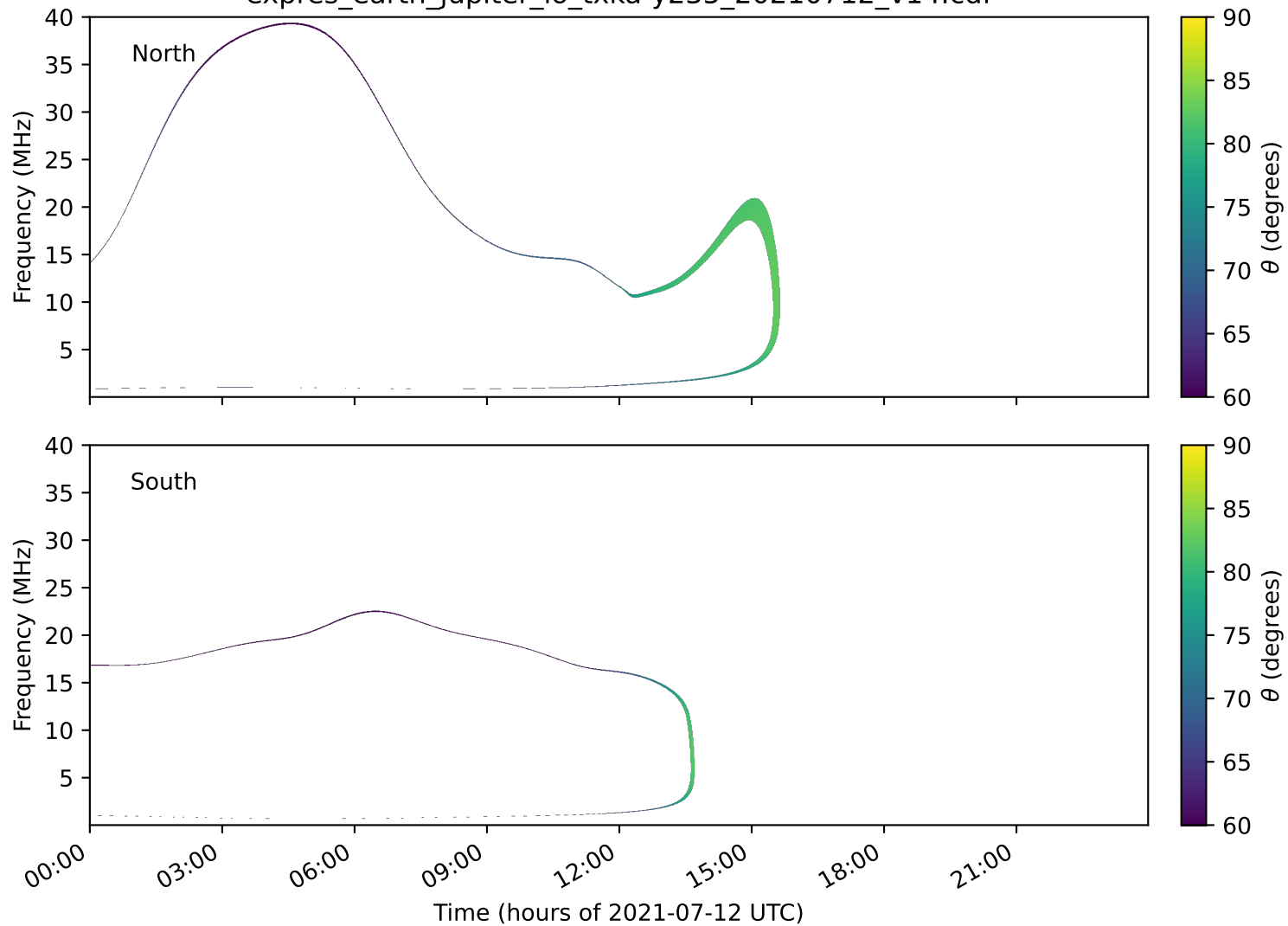
expres_earth_jupiter_io_txka-y235_20210712_v14.cdf
