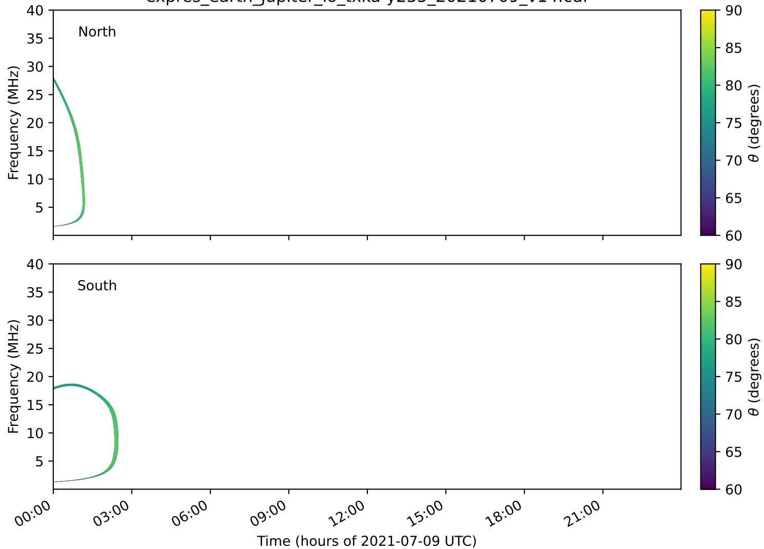
expres_earth_jupiter_io_txka-y235_20210709_v14.cdf
