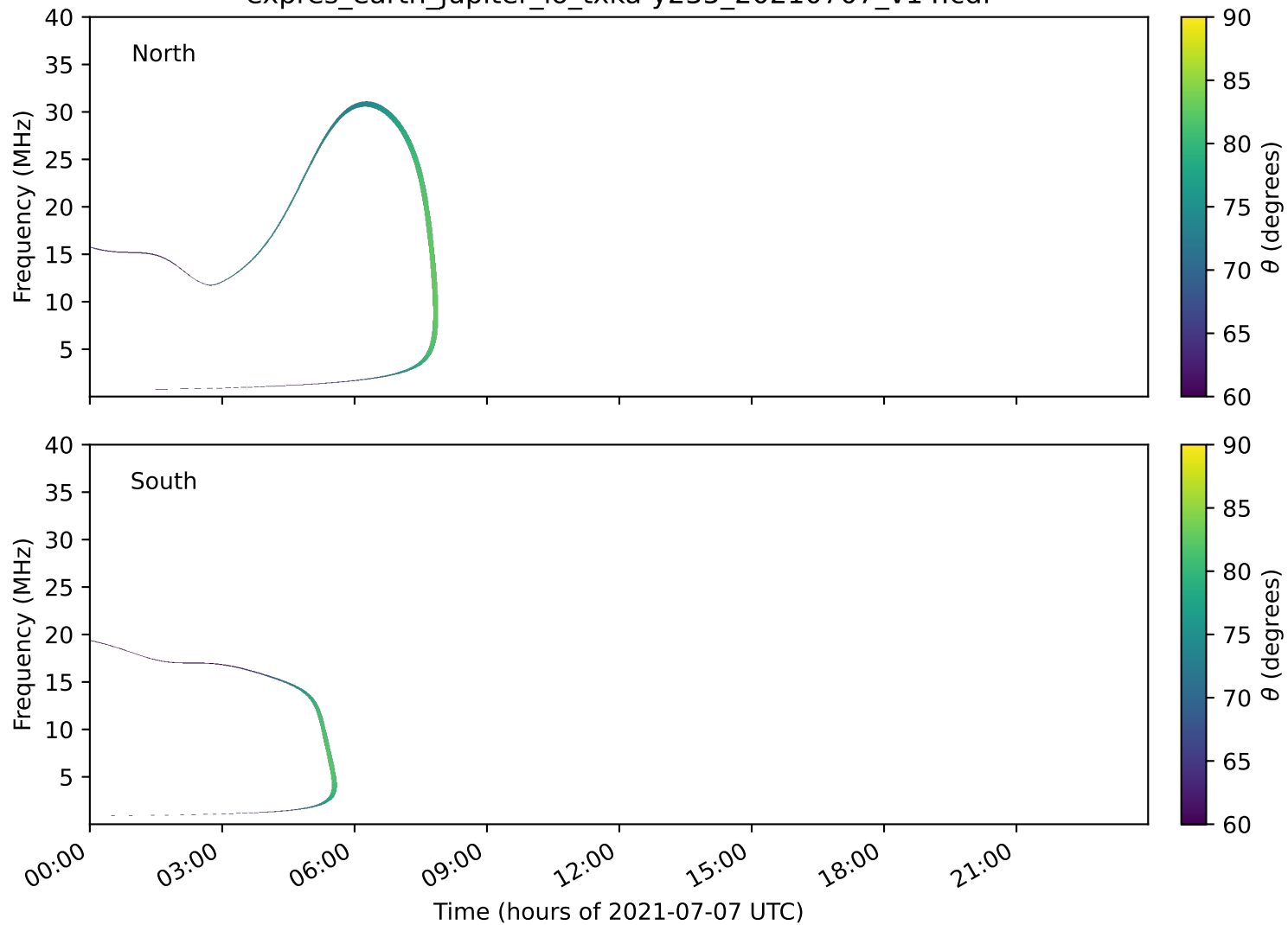
expres_earth_jupiter_io_txka-y235_20210707_v14.cdf
