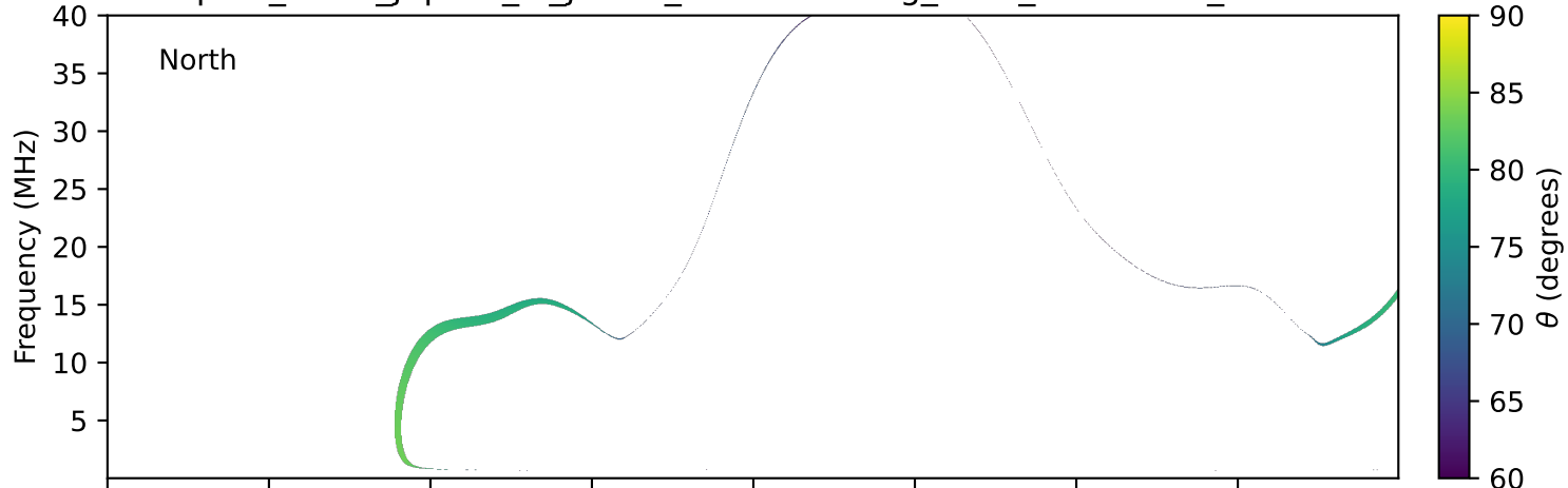
expres_earth_jupiter_io_jrm33_lossc-wid1deg_3kev_20210731_v11.cdf
