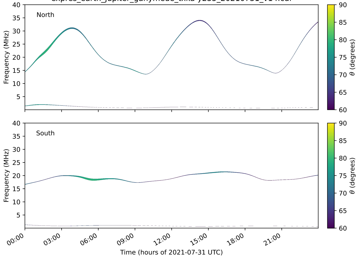
expres_earth_jupiter_ganymede_txka-y235_20210731_v14.cdf
