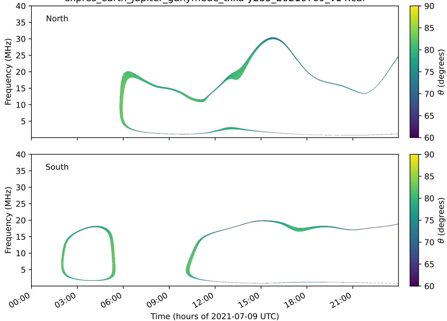
expres_earth_jupiter_ganymede_txka-y235_20210709_v14.cdf
