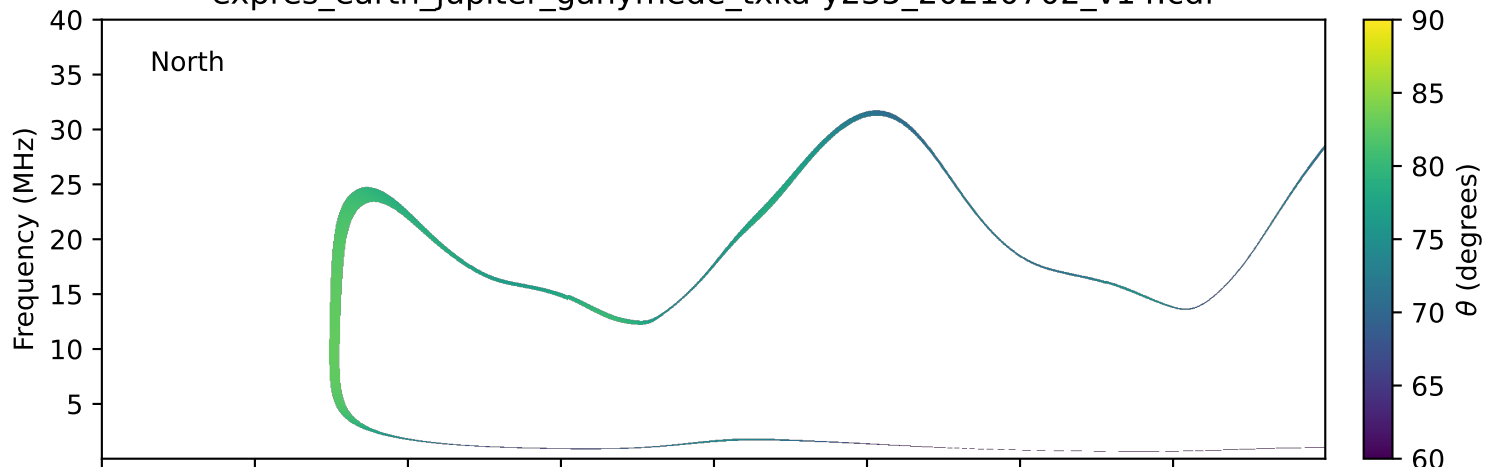
expres_earth_jupiter_ganymede_txka-y235_20210702_v14.cdf
