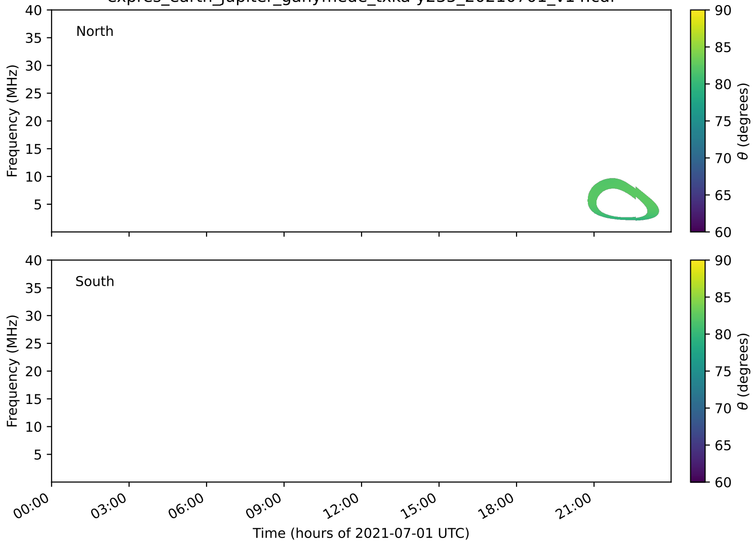
expres_earth_jupiter_ganymede_txka-y235_20210701_v14.cdf
