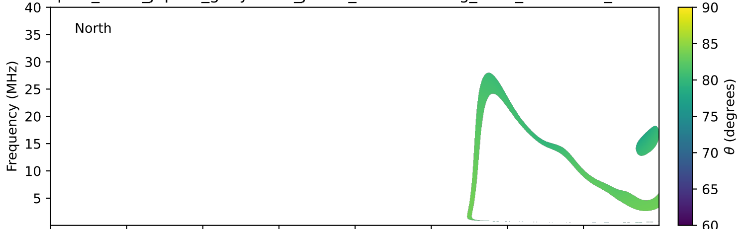
expres_earth_jupiter_ganymede_jrm33_lossc-wid1deg_3kev_20210723_v11.cdf
