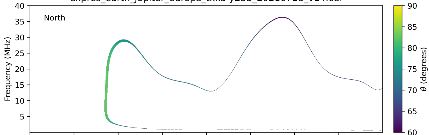
expres_earth_jupiter_europa_txka-y235_20210728_v14.cdf
