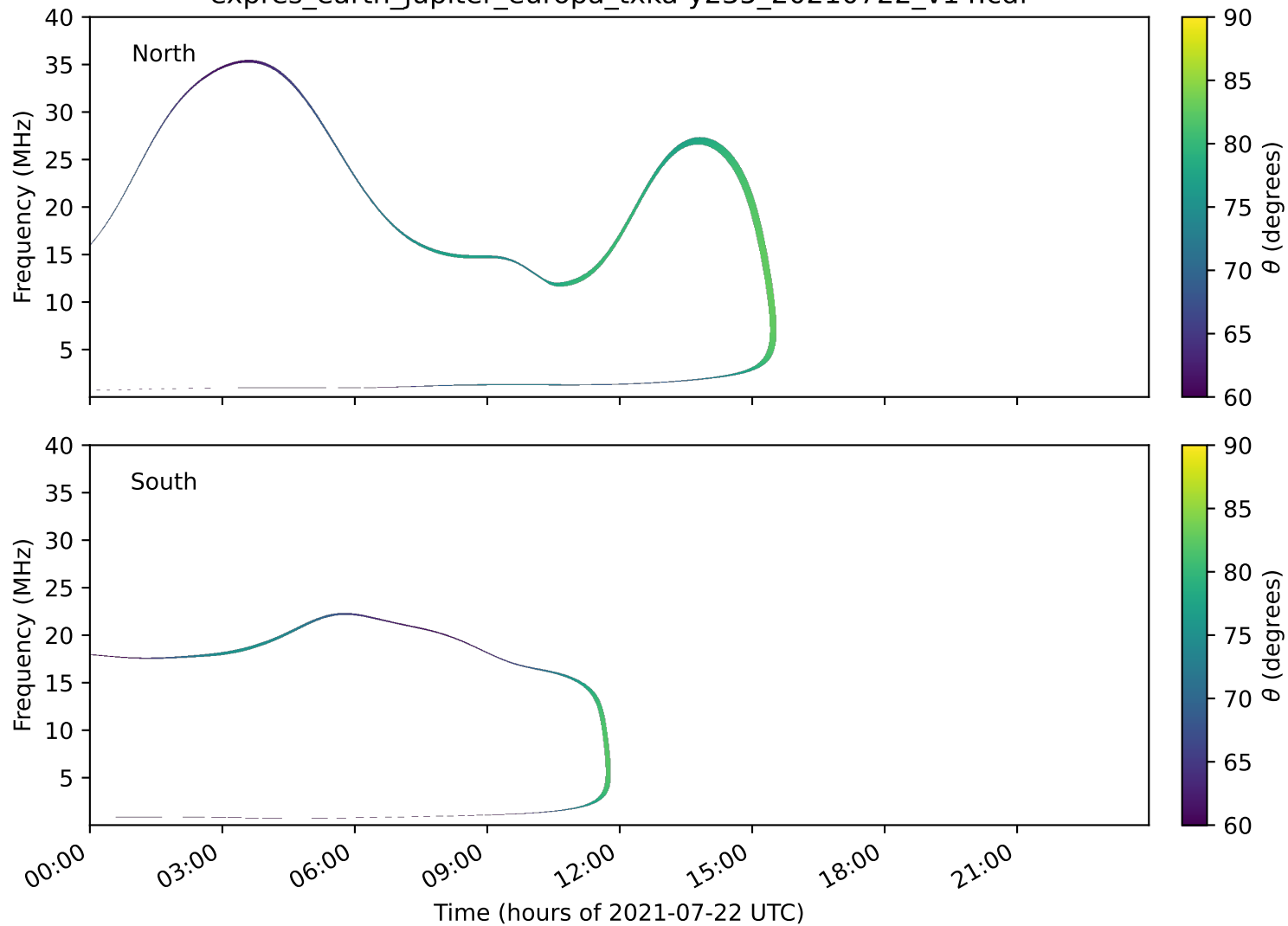
expres_earth_jupiter_europa_txka-y235_20210722_v14.cdf
