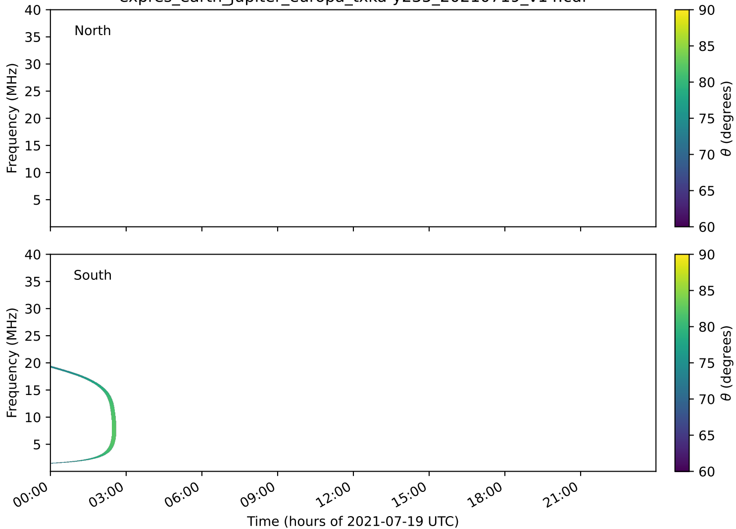
expres_earth_jupiter_europa_txka-y235_20210719_v14.cdf
