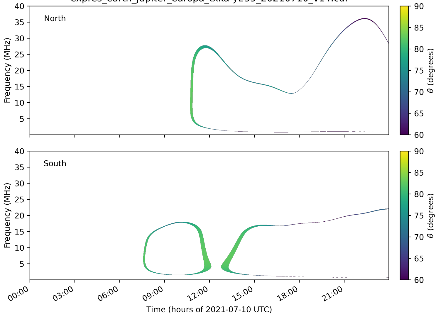
expres_earth_jupiter_europa_txka-y235_20210710_v14.cdf
