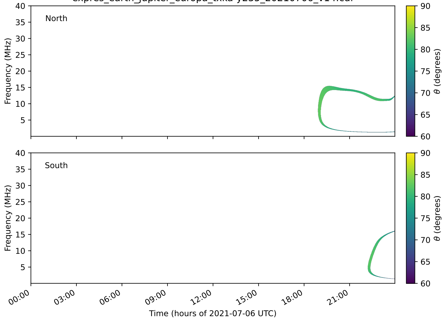
expres_earth_jupiter_europa_txka-y235_20210706_v14.cdf
