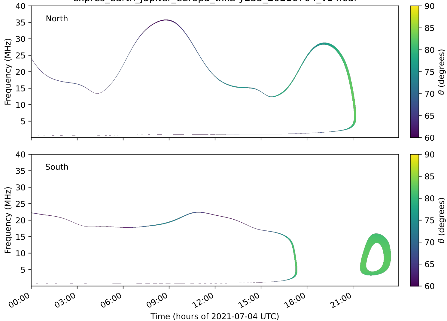
expres_earth_jupiter_europa_txka-y235_20210704_v14.cdf
