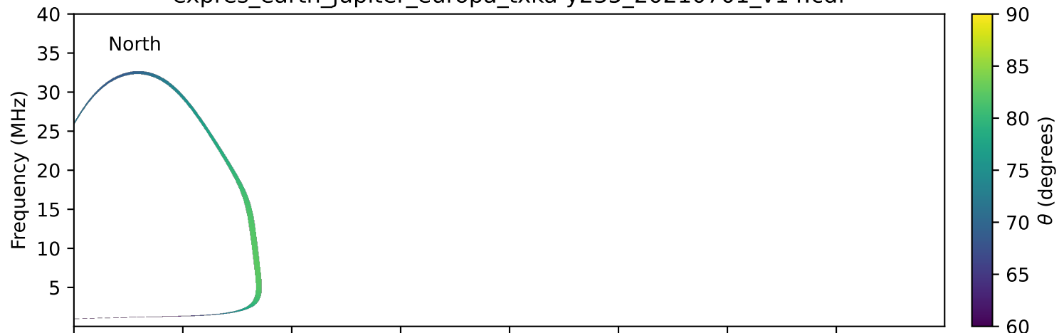
expres_earth_jupiter_europa_txka-y235_20210701_v14.cdf
