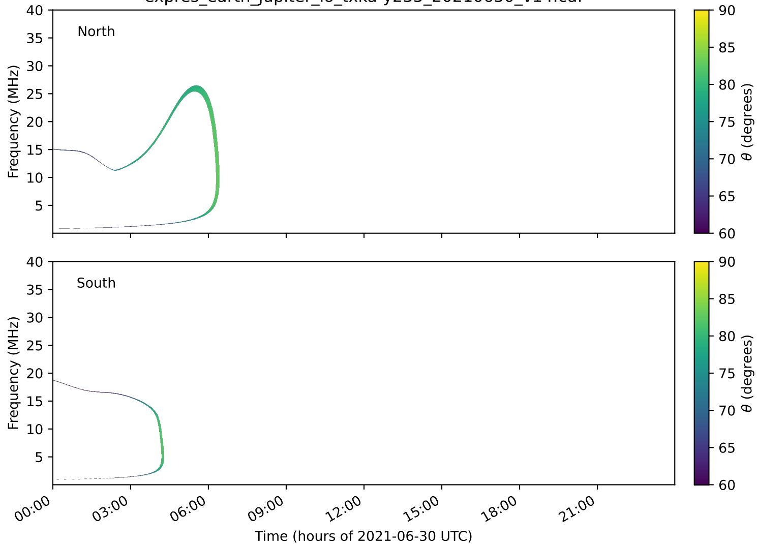
expres_earth_jupiter_io_txka-y235_20210630_v14.cdf
