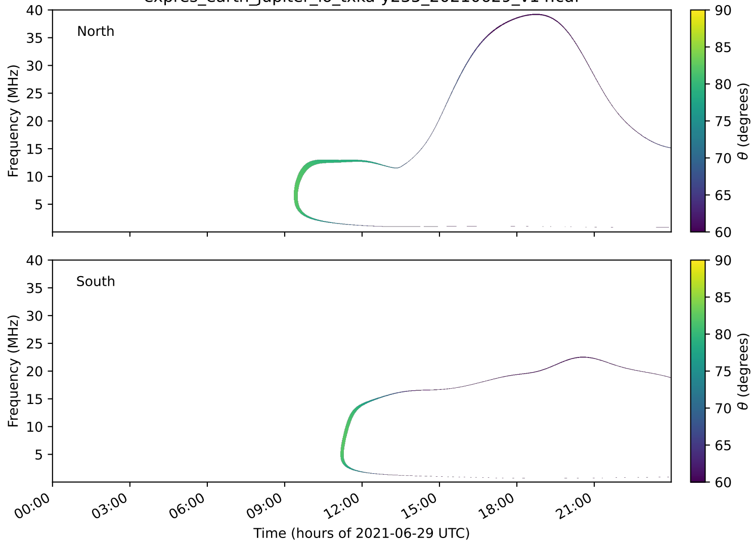
expres_earth_jupiter_io_txka-y235_20210629_v14.cdf
