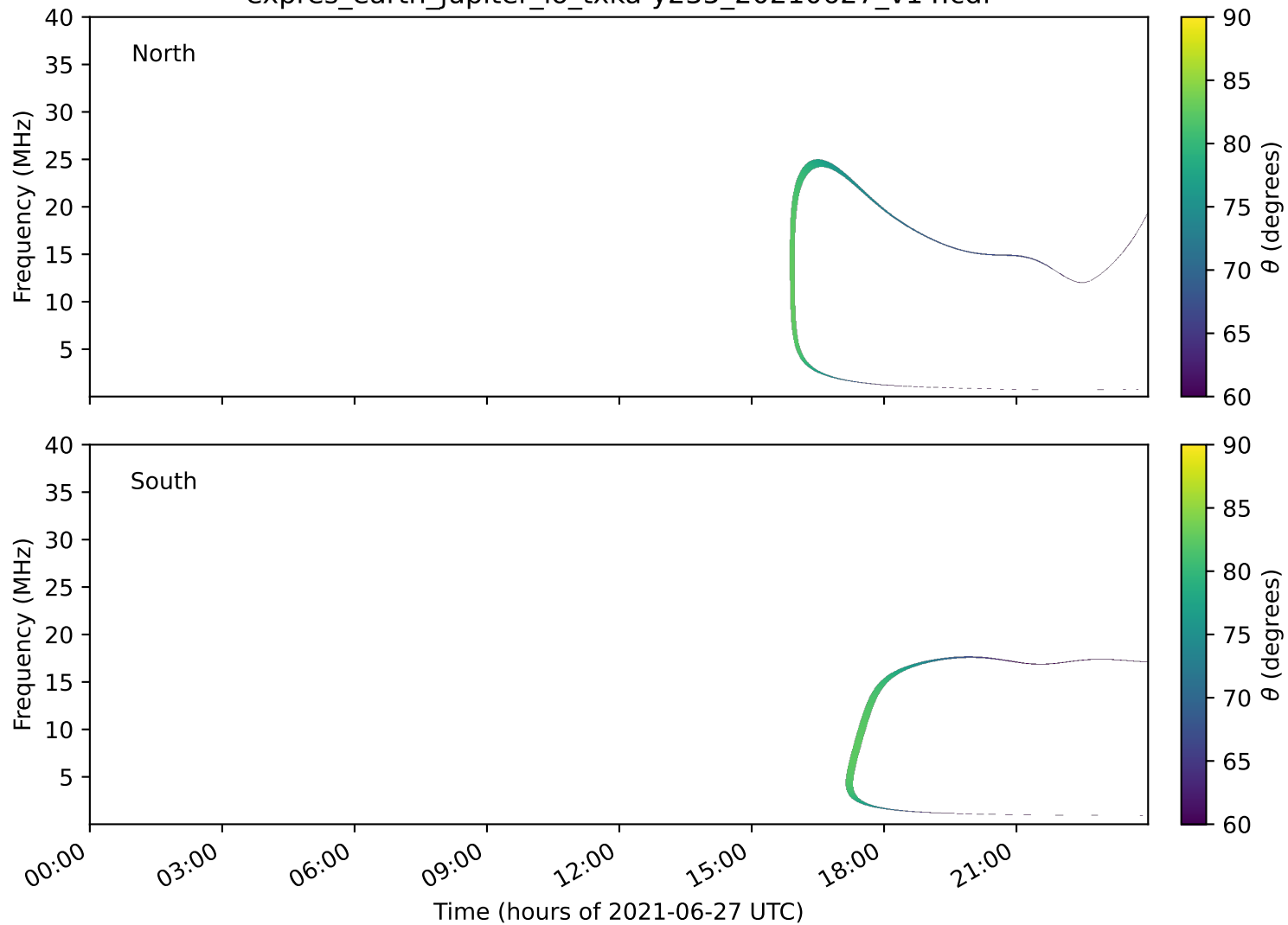
expres_earth_jupiter_io_txka-y235_20210627_v14.cdf
